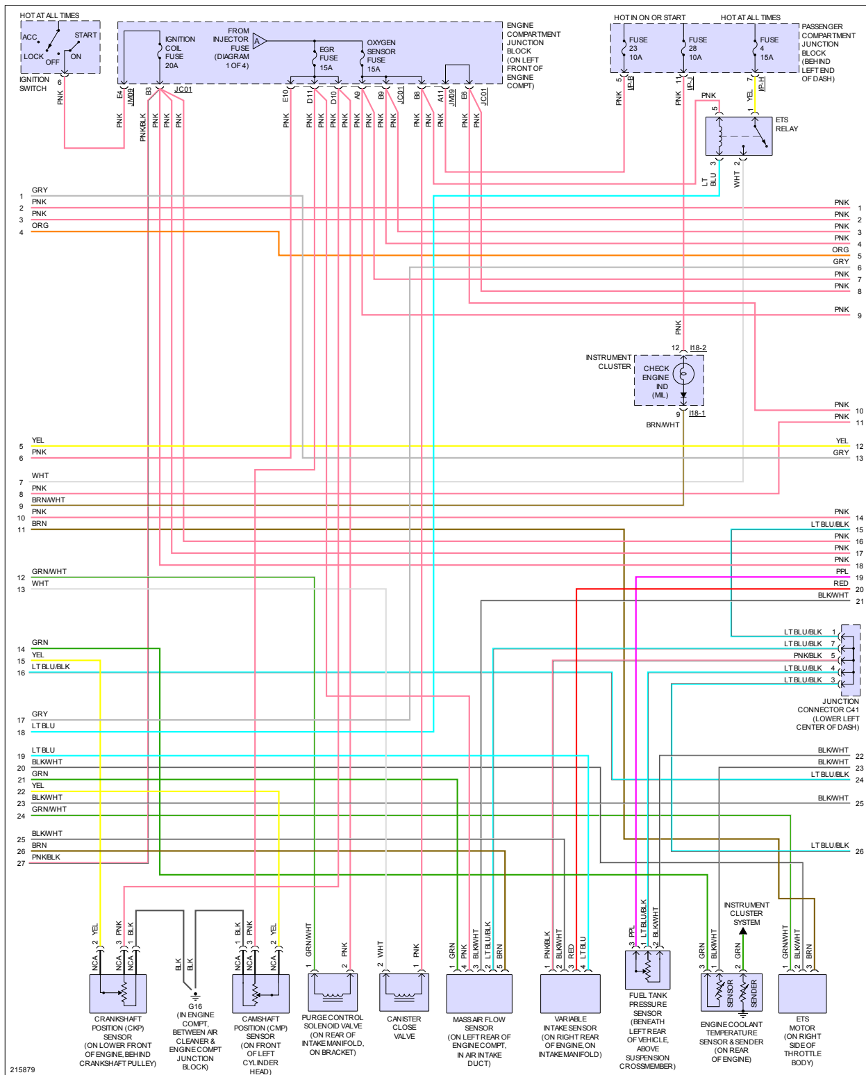
Fig 2: 3.5L, Engine Performance Circuit (2 of 4)
