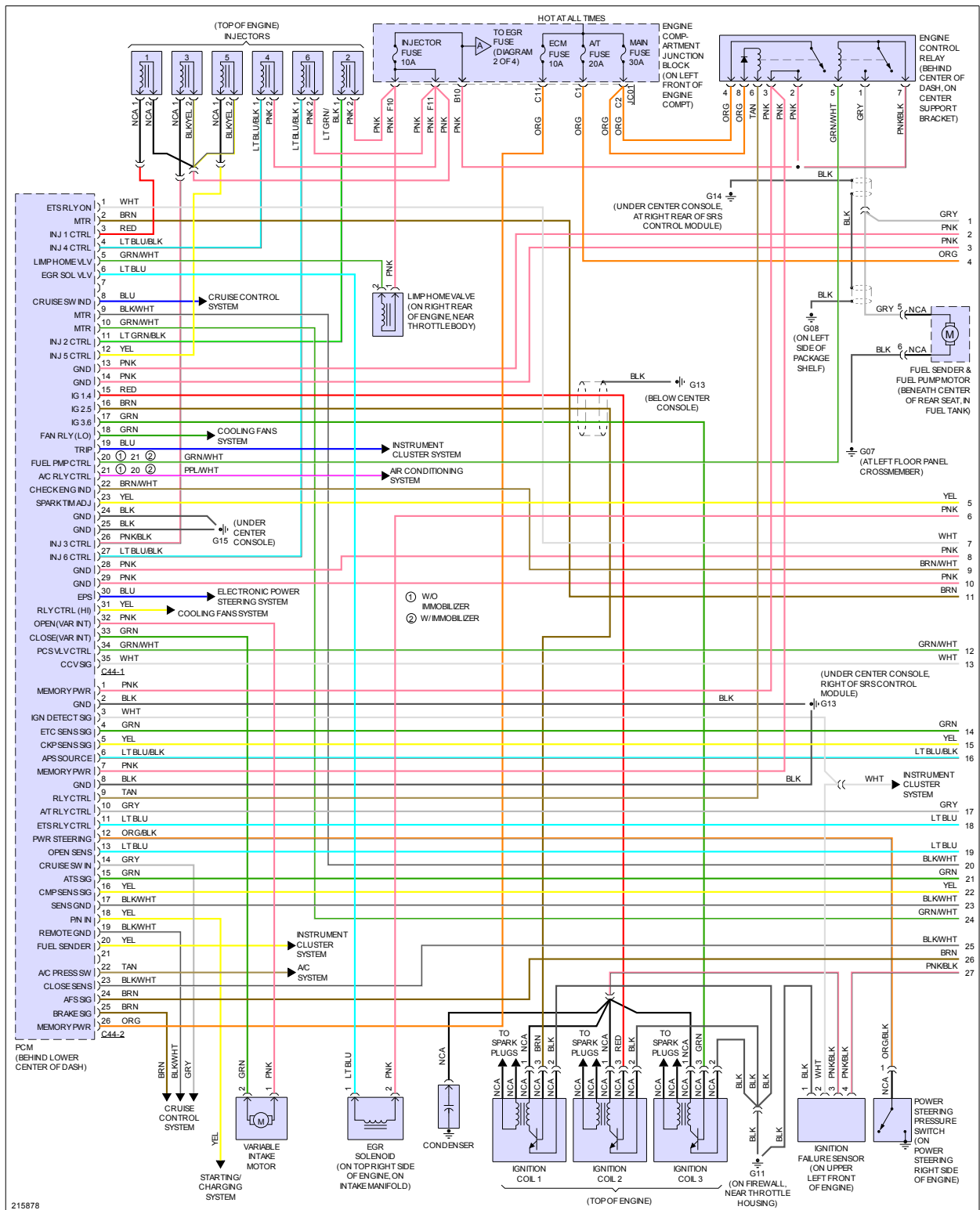
Fig 1: 3.5L, Engine Performance Circuit (1 of 4)
