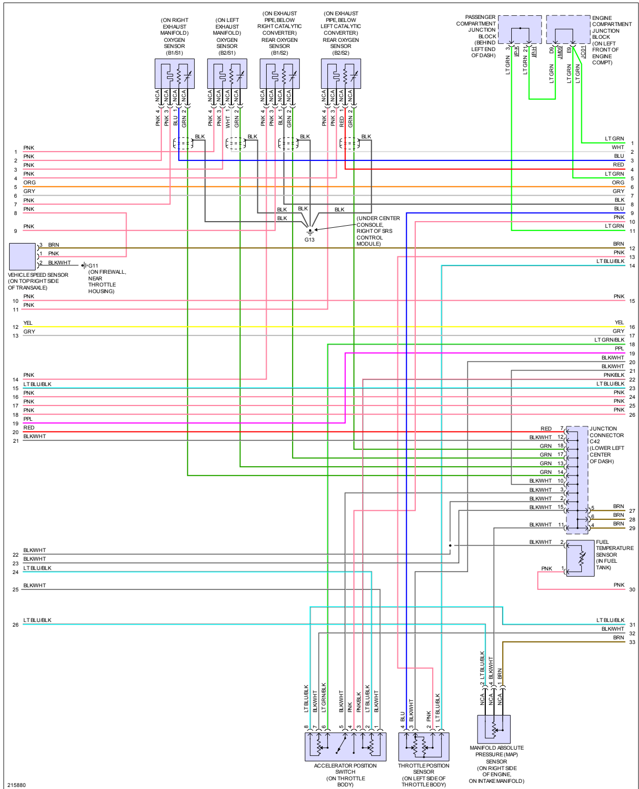
Fig 3: 3.5L, Engine Performance Circuit (3 of 4)
