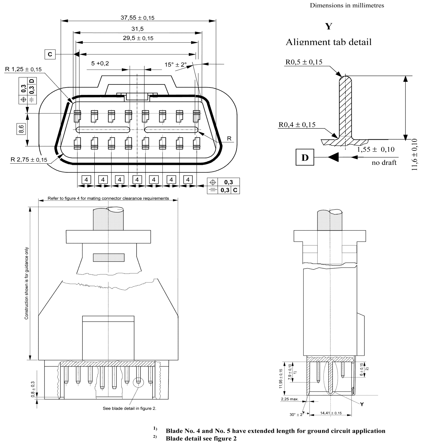
FIGURE B2—EXTERNAL TEST EQUIPMENT CONNECTOR TYPE B
